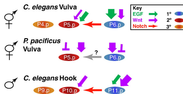
Fig. 7. Comparison of VPC and HCG patterning networks in C. elegans and Pristionchus pacificus . In the C. elegans hermaphrodite, the EGF signal is produced by the anchor cell and induces the 1° VPC fate. The Wnt pathway is required for VPC competence and has a minor role in induction. In the C. elegans male, the EGF and Wnt pathways participate in HCG specification. However, the relative contributions of these two pathways in hook development are likely different from their contributions in vulval development, as Wnt signaling plays a relatively major role in this process. In response to a high level of Wnt and EGF signal(s), the LIN-17 and LET-23 receptors, respectively, on the cell surface of P11.p activate downstream pathways to specify the 1° fate, which produces ligands (DSL) for LIN-12/Notch. In P10.p, activated LIN-12/Notch signaling by the adjacent 1° P11.p cell acts with a weak Wnt and/or EGF signal to promote the 2° HCG fate. P9.p receives little (if any) signal, and therefore usually fuses with hyp7 , adopting a 3° fate. In P. pacificus , different Wnt ligands act to induce as well as inhibit vulval development. A lateral signal from P6.p induces P5.p and P7.p. to adopt the 2° fates. It is not known if this is mediated by LIN-12/Notch.
